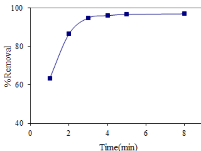
Figure 8. Effect of contact time of removal MB on \text{Fe}_3\text{O}_4@\text{MCM-41}@\text{MAA-APTES}
