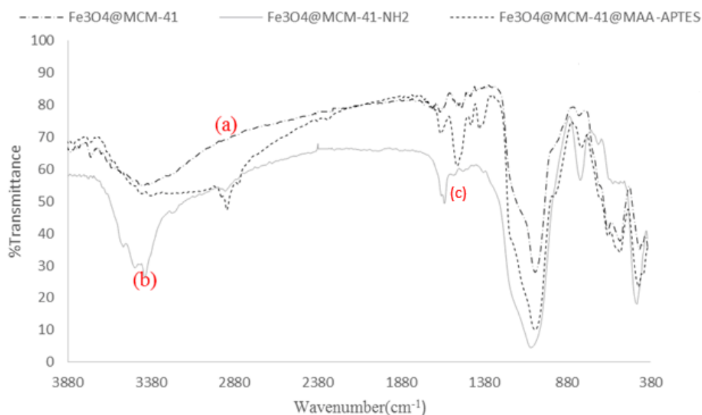
Figure 3. FT-IR spectra of synthesis magnetic mesoporous silica
