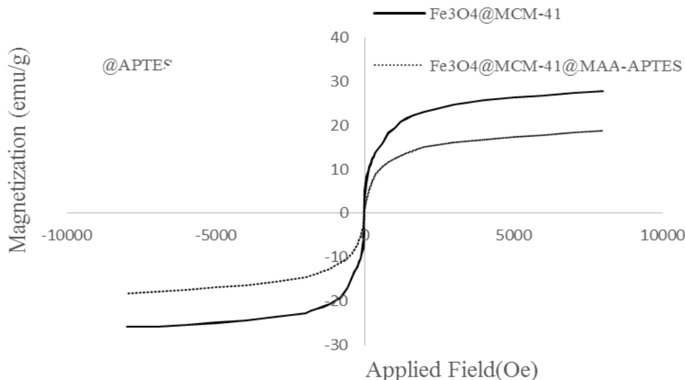
Figure 5. Magnetic curves of the \text{Fe}_3\text{O}_4@\text{MCM-41} (—) and \text{Fe}_3\text{O}_4@\text{MCM-41}@\text{MAA-APTES} (.....)
