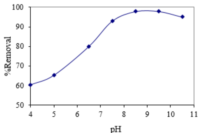
Figure 6. Effect of pH on the removal of MB at room temperature \text{Fe}_3\text{O}_4@\text{MCM-41}@\text{MAA-APTES}
