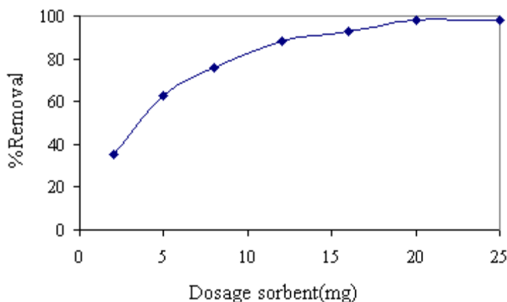
Figure 7. Effect of amount of adsorbent (g) on MB removal at room temperature by \text{Fe}_3\text{O}_4@\text{MCM-41}@\text{MAA-APTES}
