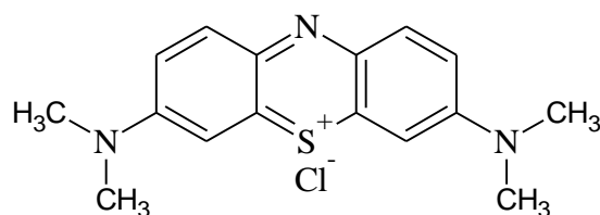
Figure 1. Chemical structure of MB
