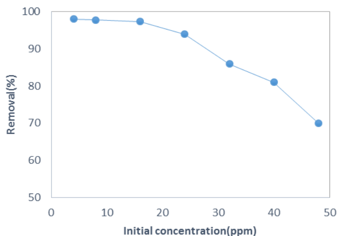
Figure 9. The effect of initial MB concentration on percent removal
