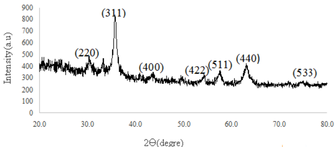
Figure 2. XRD pattern of Fe_3O_4@MCM-41@MAA-APTES
