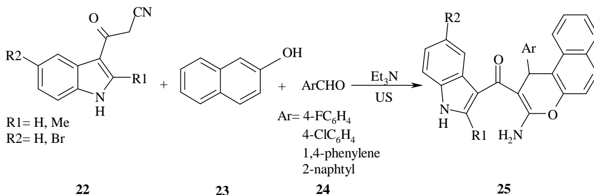
Scheme 5. 1H-benzo[f]chromen-2-yl(1H-indol-3-yl)methanones synthesis
