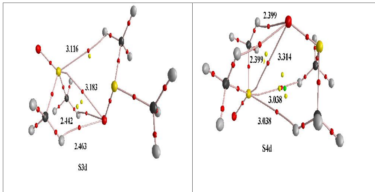
Figure 2. Molecular graph of the dimer minima obtained at the M05-2x/aug-cc-pVDZ computational level. The red and yellow dots represent the position of the bond and ring critical points, respectively. The interatomic distances ( \text{\AA} ) of those atoms that shows intermolecular interactions.
