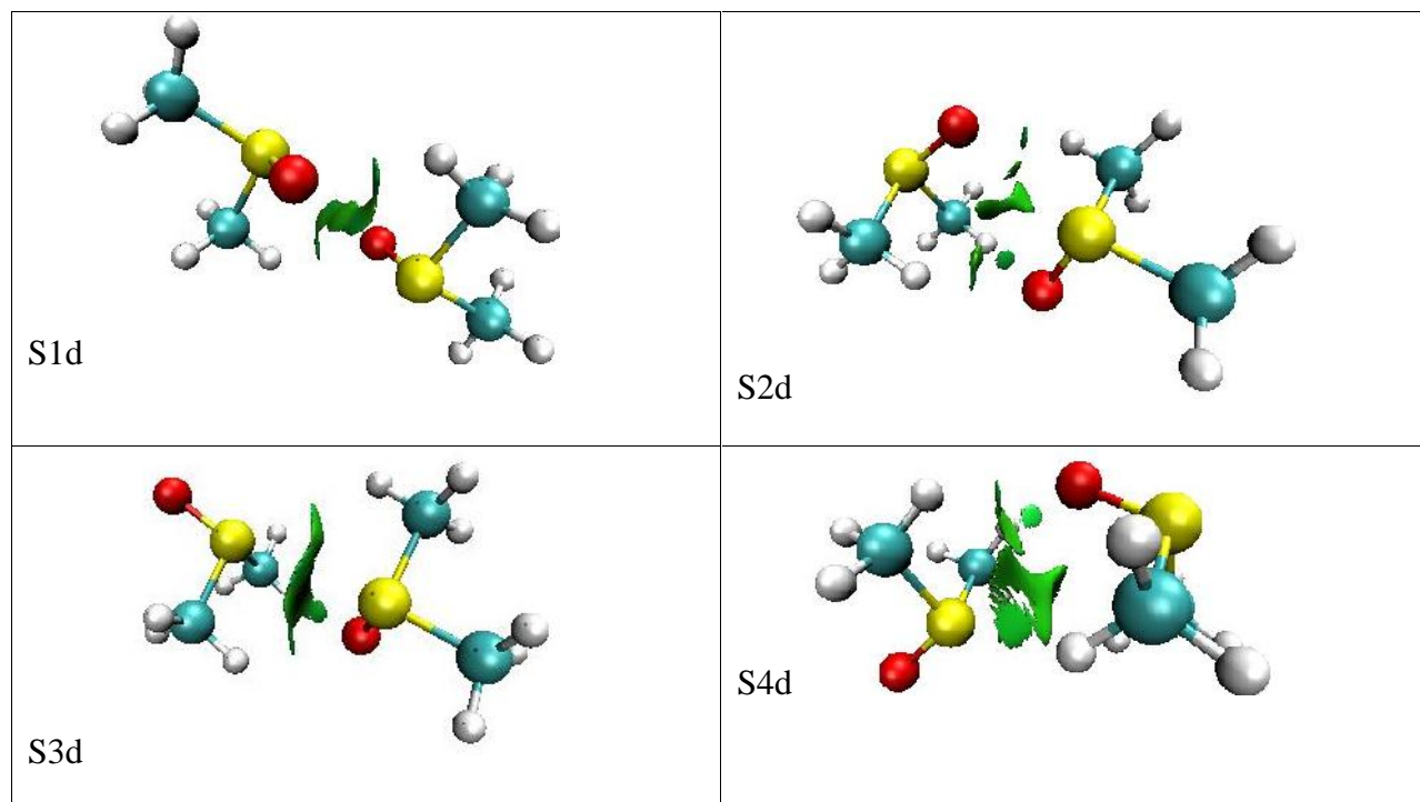
Figure 3. Noncovalent region between interacting atoms in complexes pairing DMSO molecules
