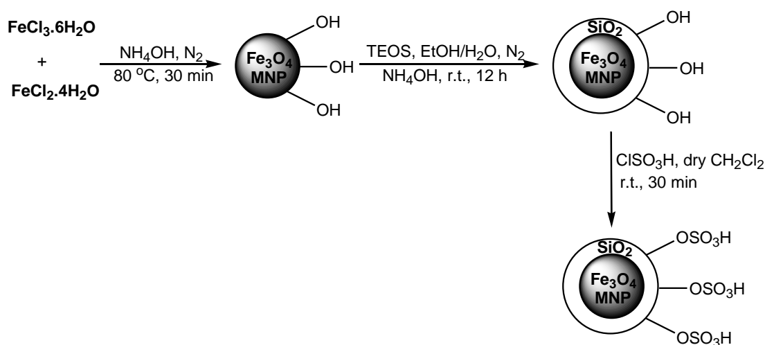
Scheme 2. Schematic diagram for the preparation of Fe 3 O 4 @SiO 2 -SO 3 H
