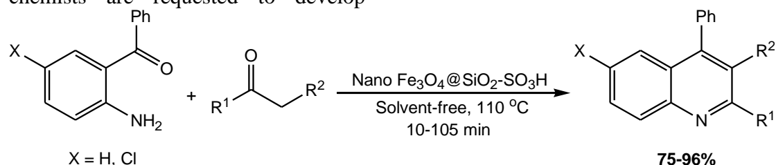
Scheme 1. Friedländer reaction of 2-aminoaryl ketones with carbonyl compounds containing \alpha -methylene groups
