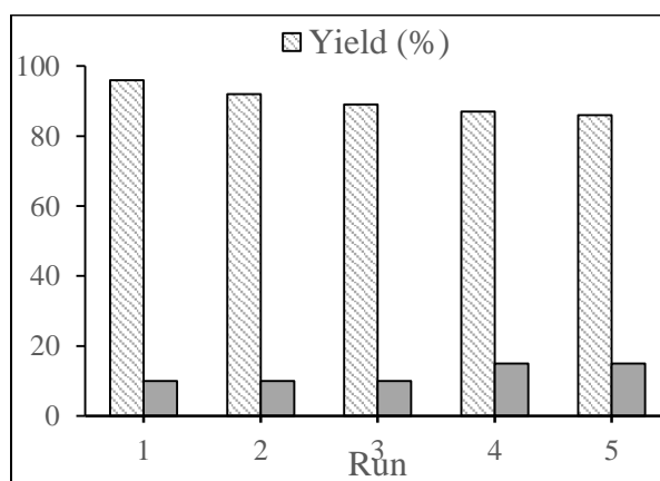
Figure 2. Reusability of the catalyst in the reaction of 2-amino-5-chlorobenzophenone (1.0 mmol) with dimedone (1.2 mmol) at 110 °C under solvent-free conditions
