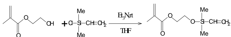
Scheme 1. Reaction of HEMA with chlorodimethylvinylsilane
