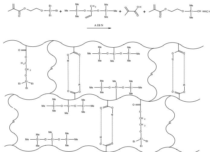
Scheme 4. Preparation of cross-linked copolymer containing siloxyl groups
