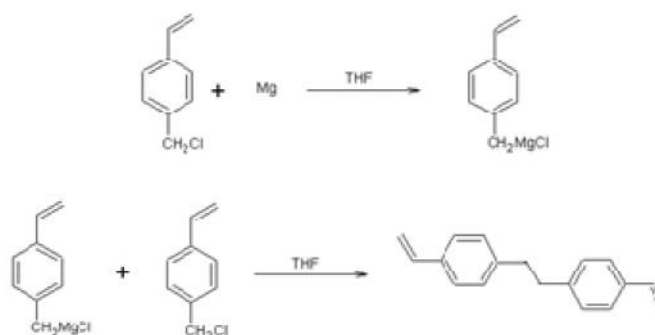
Scheme 3. The coupling reaction for preparing of BVPE (CA 2 )
