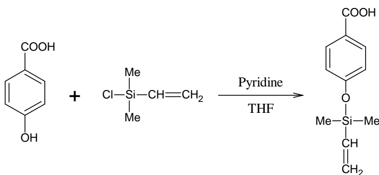
Scheme 5. Preparation of para-Dimethylvinylsiloxy-Benzoic acid
