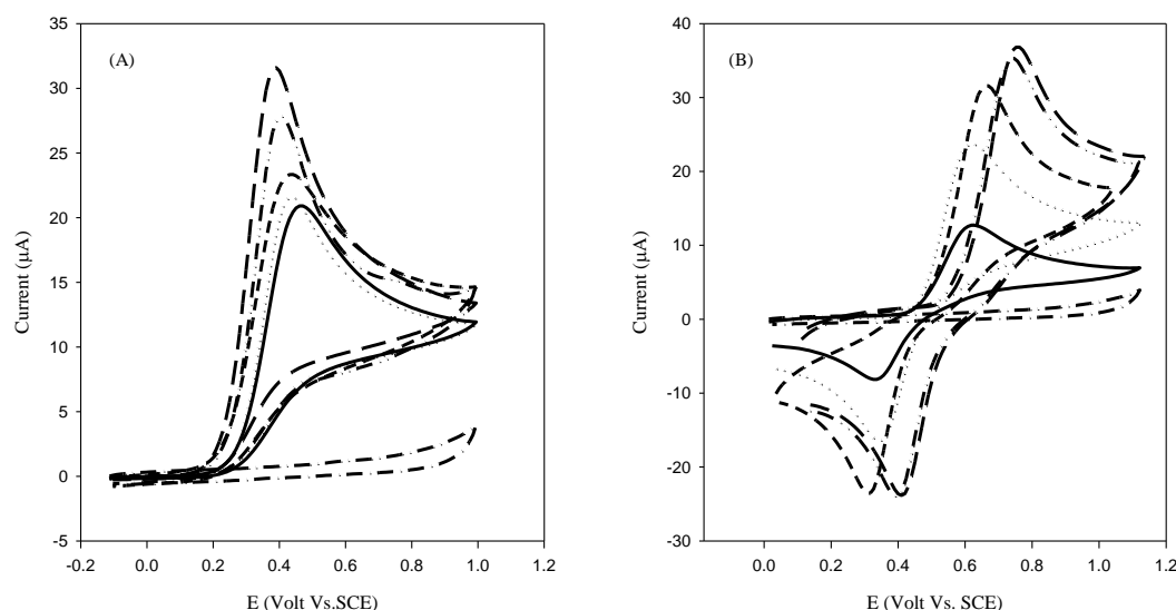
Figure 1. CV responses of blank buffered solution of pH 5.0 using cis - [\text{Mo}(\text{O})_2\text{L}] /modified CPE containing 1.5% [\text{BMIM}]\text{BF}_4 (-.-) and of 1 mM AA (A) and 1 mM DA (B) in the same buffer at the surface of unmodified CPE (—), CoL/modified CPE containing 0% (.....), 1% (---), 1.5% (-.-) and 2% [\text{BMIM}]\text{BF}_4 (---). Sweep rate: 100 \text{ mVs}^{-1} ; pulse amplitude: 50 mV.
