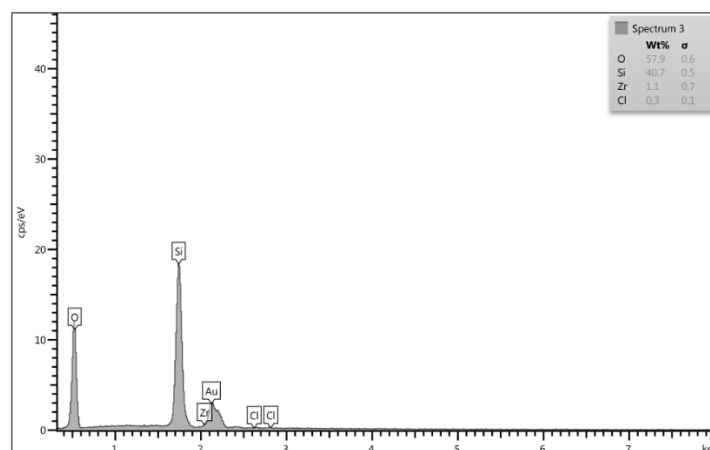
Figure 3. EDX analysis of \text{ZrOCl}_2 \cdot 8\text{H}_2\text{O}@\text{nano SiO}_2
