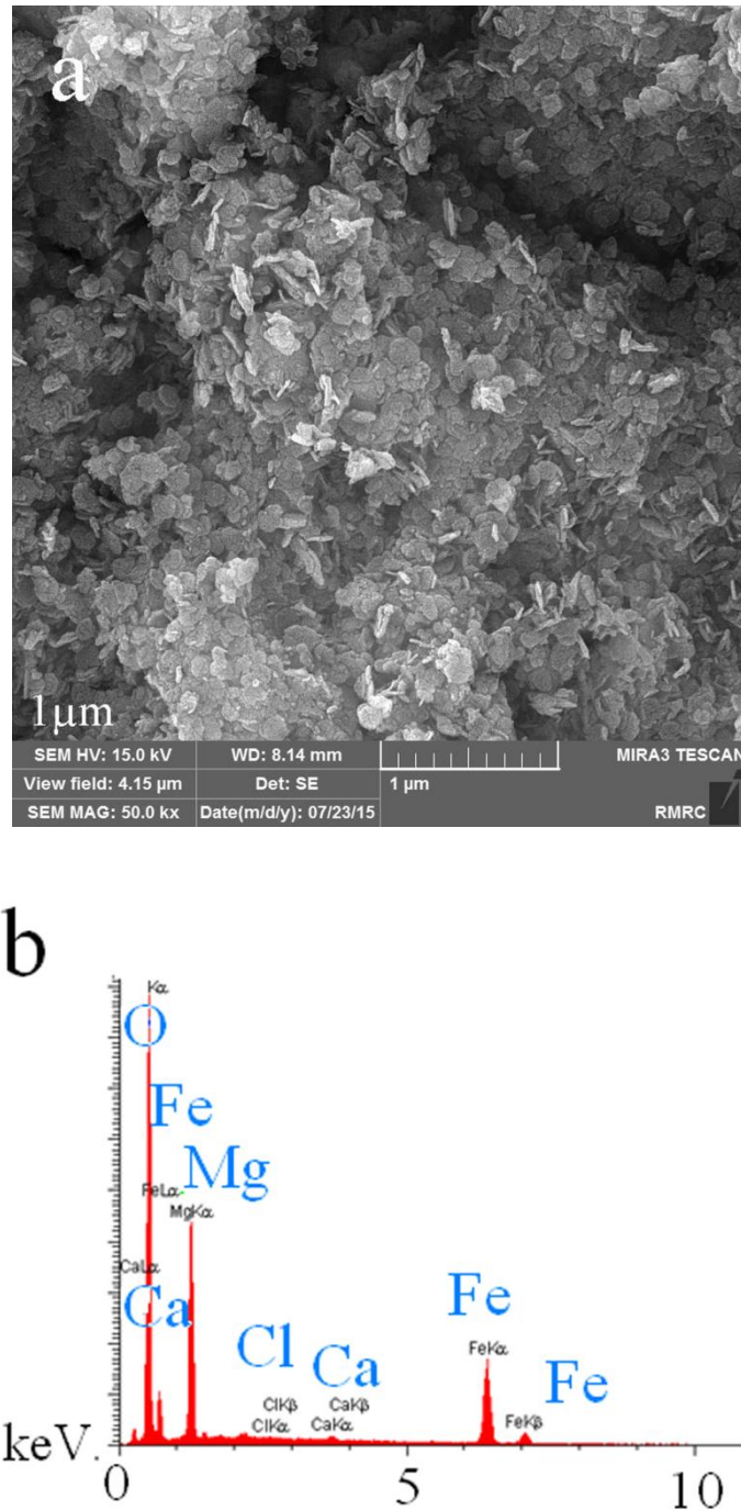
Figure 2. The SEM image (a) and EDX analysis (b) of the MgCaFe-LDH sample
