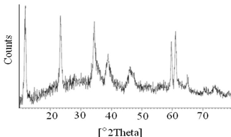
Figure 1. The XRD pattern of the MgCaFe-LDH sample
