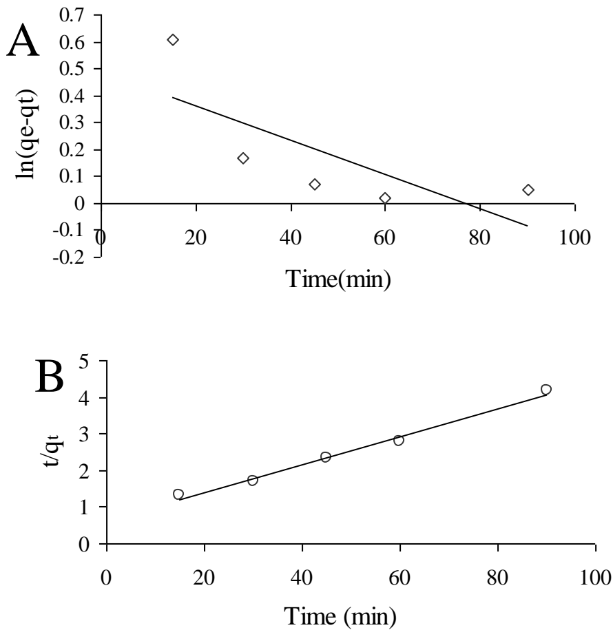
Figure 9. (A) \ln(q_e - q_t) (B) t/q_t vs time for the CR dye removal
