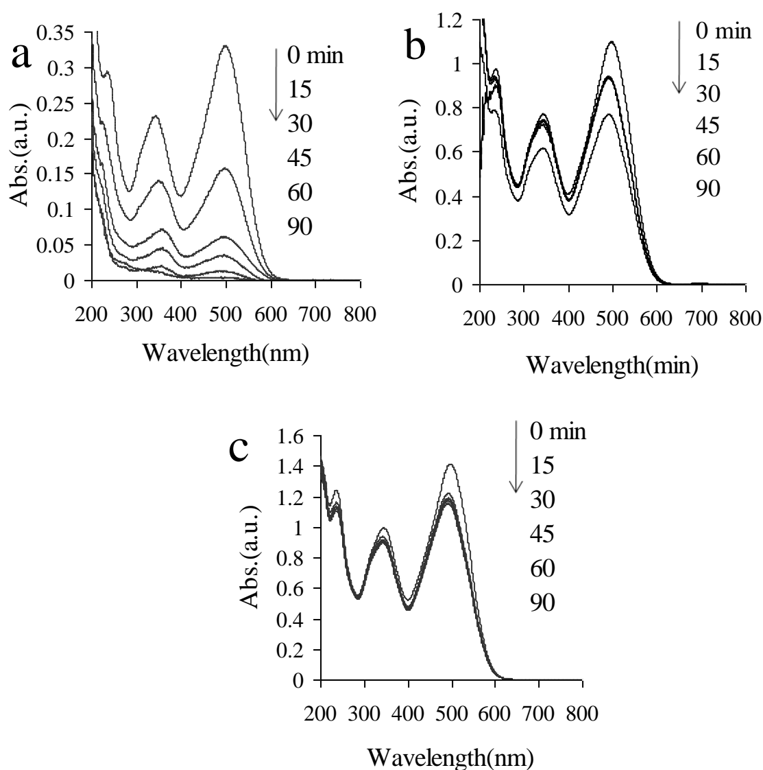
Figure 3. UV-Vis spectra changes of CR dye solutions (a) 10 \text{ mgL}^{-1} (b) 35 \text{ mgL}^{-1} and (c) 50 \text{ mgL}^{-1} during adsorption experiments on MgCaFe-LDH sample
