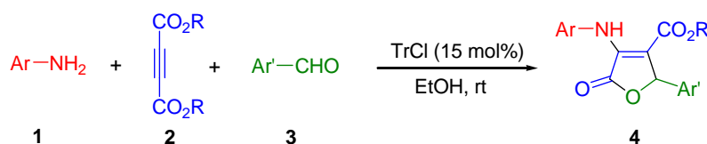
Scheme 1. Synthesis of 3-amino-2-oxofuranes 4
