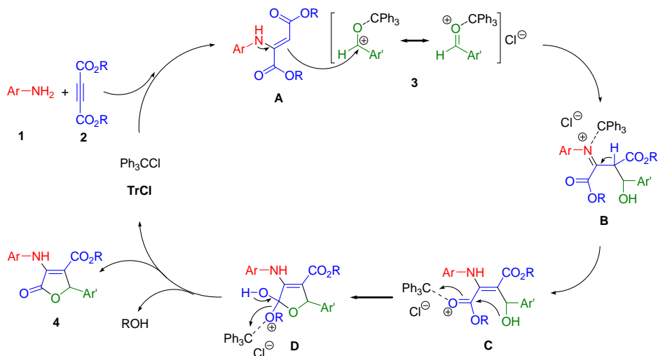
Scheme 2. Proposed mechanism for the synthesis of 2-oxofurane 4
