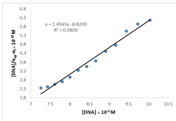
Figure 3. The plot of [ct\text{-DNA}]/(\epsilon_{app} - \epsilon_f) versus [ct\text{-DNA}]
