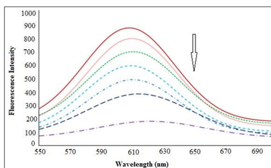
Figure 4. Emission spectra of the EB-ct-DNA complex in the presence of the increasing amounts of [\text{Ni}(\text{FIP})_2](\text{OAC})_2 complex in DNA/EB in 20 mM Tris/HCl buffer solution, pH 7 and at 25 °C
