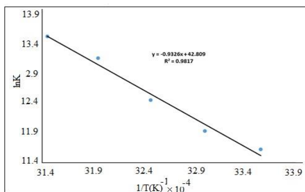
Figure 6. The van't Hoff plot [\text{Ni}(\text{FIP})_2](\text{OAC})_2 binding to ct-DNA
