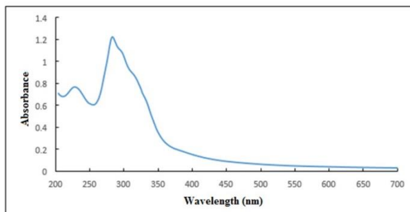
Figure 1. UV-Vis spectrum of [\text{Ni}(\text{FIP})_2](\text{OAC})_2 complex
