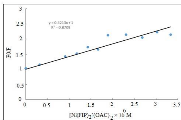
Figure 5. Plots of F_0/F versus the concentration of [\text{Ni}(\text{FIP})_2](\text{OAC})_2 complex for the binding of [\text{Ni}(\text{FIP})_2](\text{OAC})_2 with ct-DNA at room temperature
