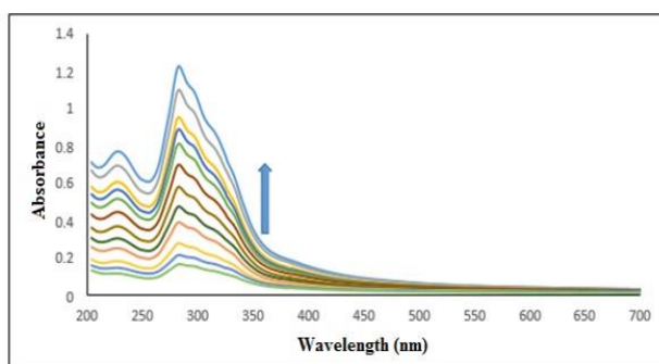
Figure 2. Absorption spectra of [\text{Ni}(\text{FIP})_2](\text{OAC})_2 ( 2 \times 10^{-5} M) upon titration with solution of ct-DNA in 20 mM Tris/HCl buffer solution, pH 7 and at 25 °C
