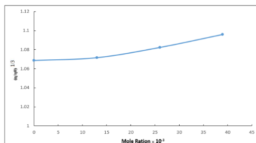
Figure 7. Relative viscosity of ct-DNA (1.35×10 -5 M) in the presence of increasing amounts of [Ni(FIP) 2 ](OAC) 2 at stoichiometric ratios R= [Ni(FIP) 2 ](OAC) 2 /[ct-DNA]=0.0-0.039, plotted as (η/η 0 ) 1/3 vs. R. Measurements were done in 20 mM Tris/HCl buffer, pH 7 and at 25 °C
