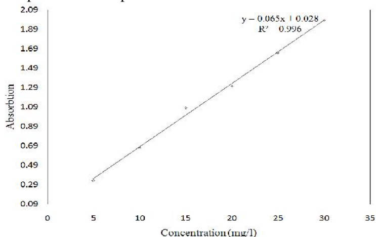
Figure 3. Calibration curve of MO
