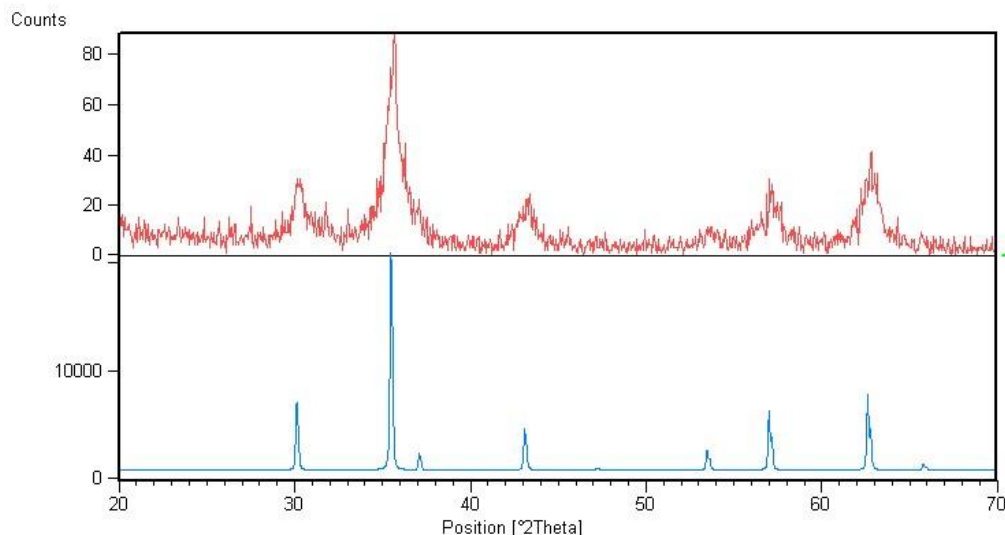
Figure 2. XRD pattern of synthesized \text{CoFe}_2\text{O}_4
