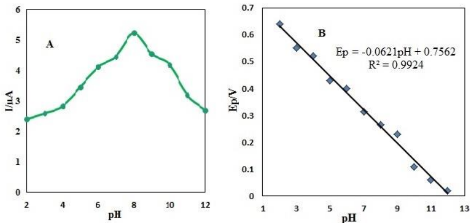
Figure 5. (A) Variation of the anodic peak current in the cyclic voltammograms of 1.0 mM DA. (B) Influence of the solution pH on the oxidation peak potential ( E_{\text{pa}} ) for 1.0 mM DA. Measurements carried out at the surface of \text{Al}_2\text{O}_3\text{NPsCPE} in 0.1M buffered solution with different pH values, 2.0, 3.0, 4.0, 5.0, 6.0, 7.0, 8.0, 9.0, 10.0, 11.0 and 12.0, at scan rate of 0.05 \text{ V s}^{-1} .
