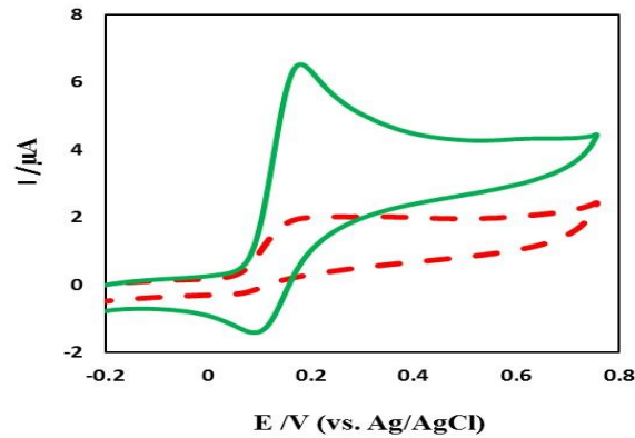
Figure 4. Cyclic voltammograms obtained for CPE (dashed line) and \text{Al}_2\text{O}_3\text{NPsCPE} (solid line) in 0.1M phosphate buffer solution of pH 8.0 containing 1.0 mM DA. Scan rate 0.1 \text{ V s}^{-1}
