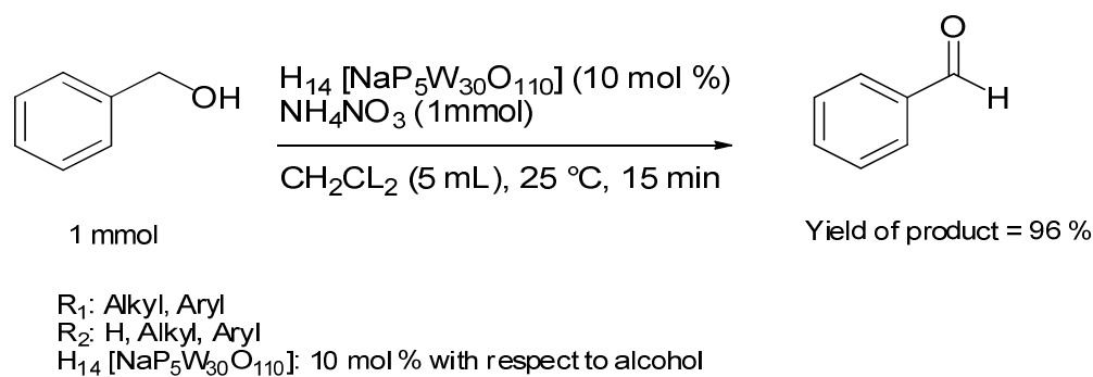
Scheme 1. Oxidation of benzyl alcohol in the presence of H 14 [NaP 5 W 30 O 110 ] and NH 4 NO 3 as green system.
