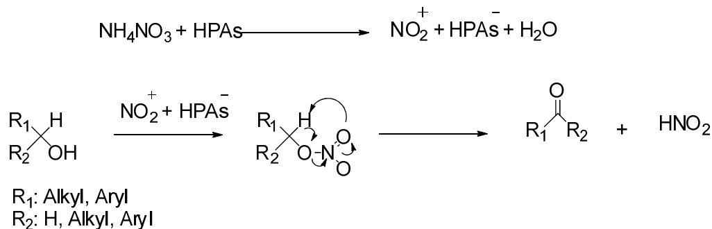
Scheme 3. Proposed mechanism for the oxidation of alcohols in the presence of NO 2 +
