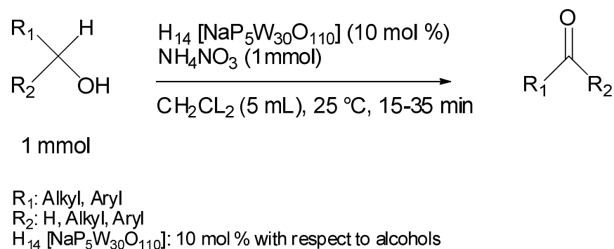
Scheme 2. Oxidation of various alcohols in the presence of H 14 [NaP 5 W 30 O 110 ] and NH 4 NO 3 as green system
